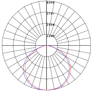
Vertical Plane Through: 0 - 90 Horizontal Horizontal Cone Through: 4 Vertical Maximum Candela = 4996.45 at 0 H 4 V
