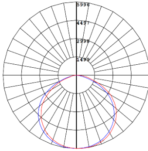
Vertical Plane Through: 0 - 90 Horizontal Horizontal Cone Through: 4 Vertical Maximum Candela = 5995.72 at 0 H 4 V
