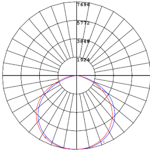
Vertical Plane Through: 0 - 90 Horizontal Horizontal Cone Through: 4 Vertical Maximum Candela = 7695.89 at 0 H 4 V
