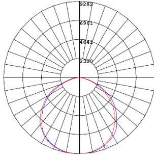
Vertical Plane Through: 0 - 90 Horizontal Horizontal Cone Through: 4 Vertical Maximum Candela = 9287.92 at 0 H 4 V
