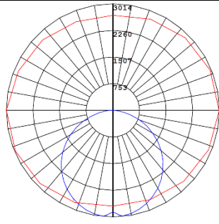
Vertical Plane Through: 180 - 0 Horizontal Horizontal Cone Through: 5 Vertical Maximum Candela = 3013.74 at 0 H 5 V
