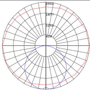
Vertical Plane Through: 180 - 0 Horizontal Horizontal Cone Through: 5 Vertical Maximum Candela = 2502.39 at 180 H 5 V
