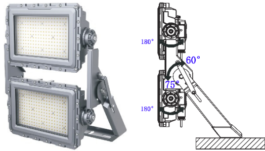
BRM – MULTI-PIVOT BRACKET
