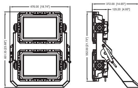
BRM – MULTI-PIVOT BRACKET
