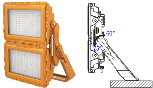
BRK - BRACKET
